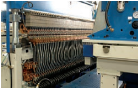
Welding machine mesh feed system (above) and machine's welding portal (below) ...36
