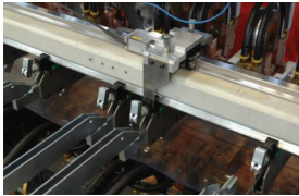
Measurement system for positioning mesh welder wire lines...42
