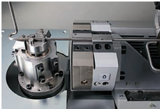
Tooling arranged for optimized bending operations ...32
